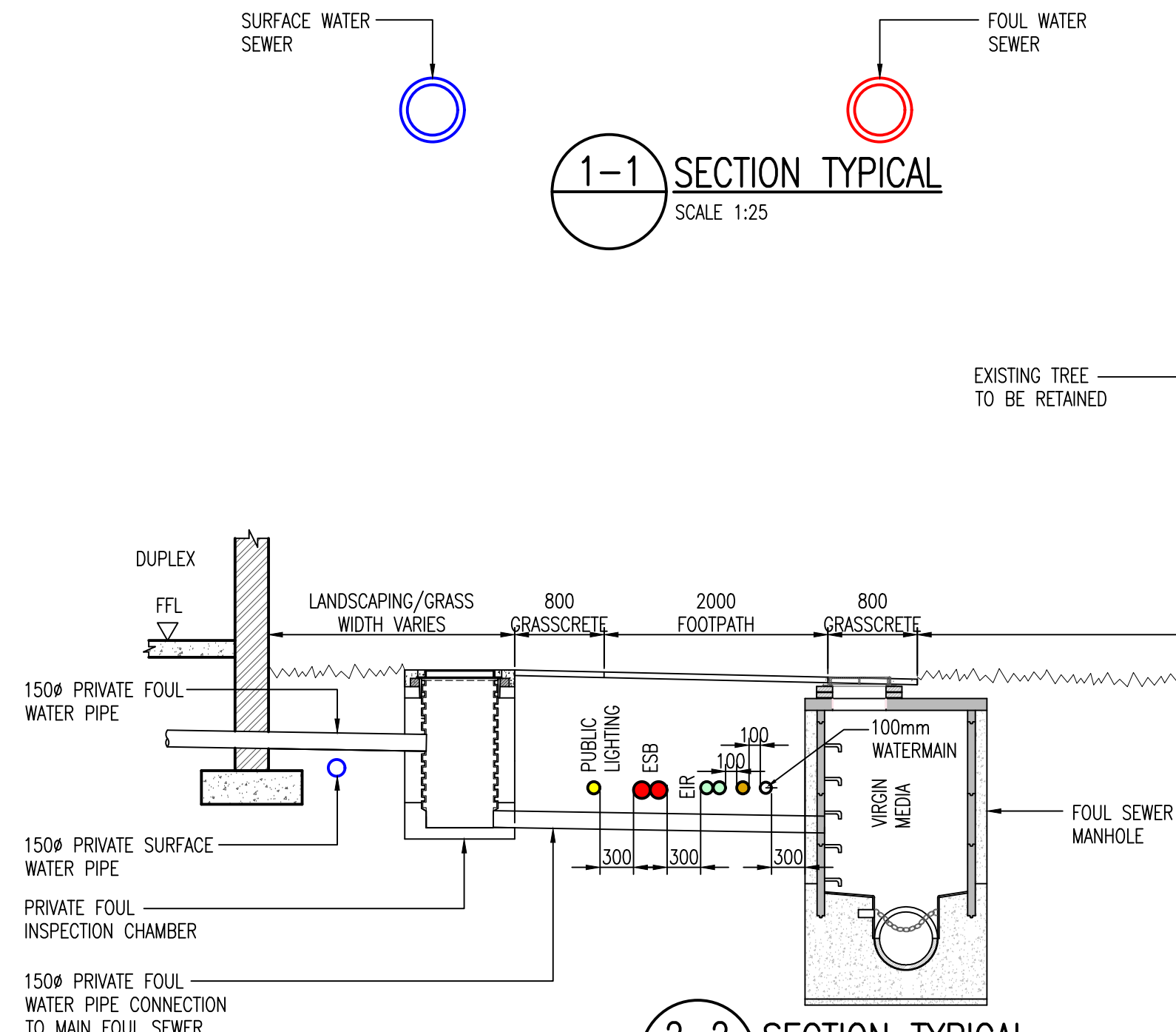
2-2 SECTION TYPICAL SCALE 1:50
